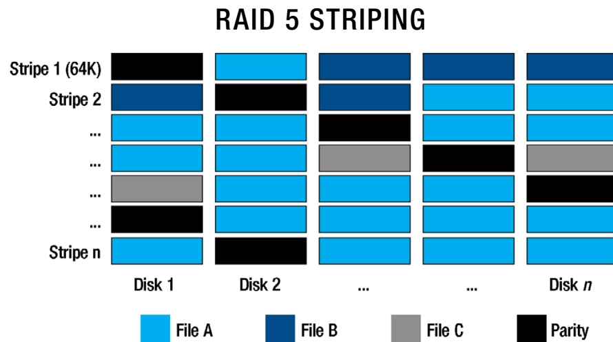
Figure1.4: 1MB "File A" unevenly written as simultaneous I/O writes are coalesced
