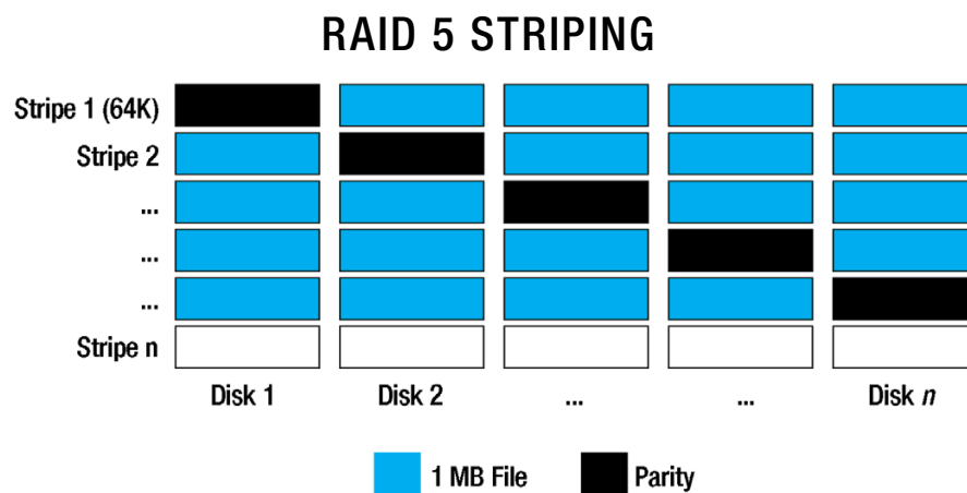
Figure1.3: 1MB file in one logical I/O, evenly striped (w/parity) across 5 disks
